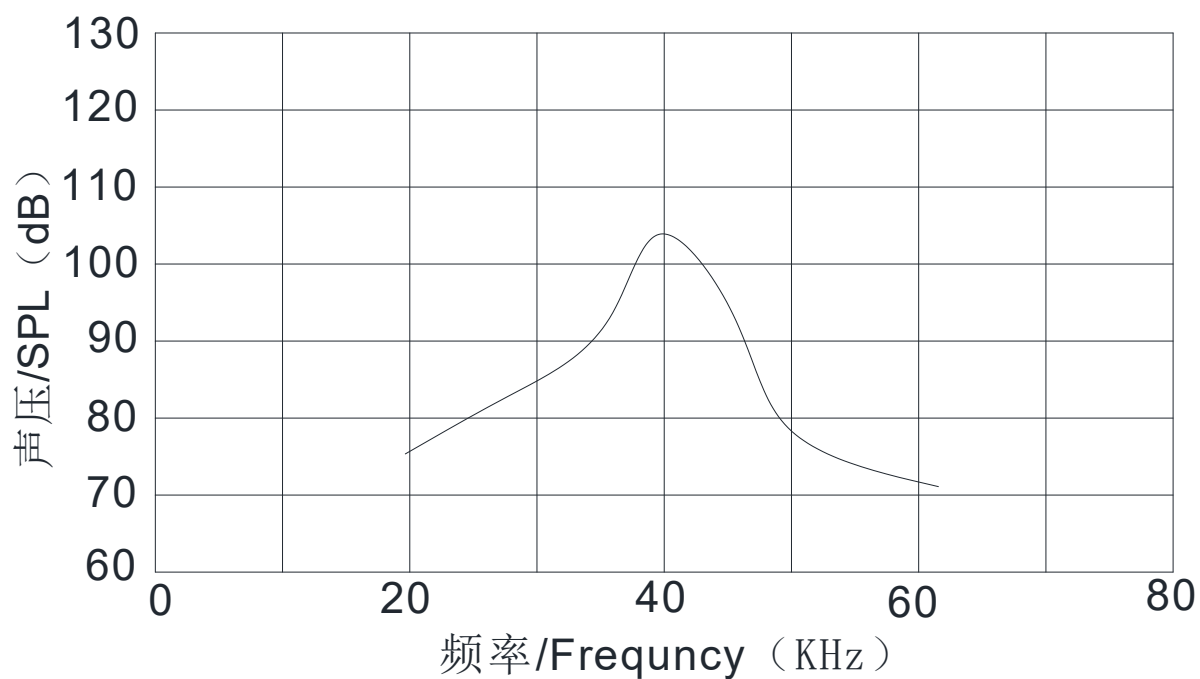
声压-频率特性曲线图/SPL-Freq.characteristics
